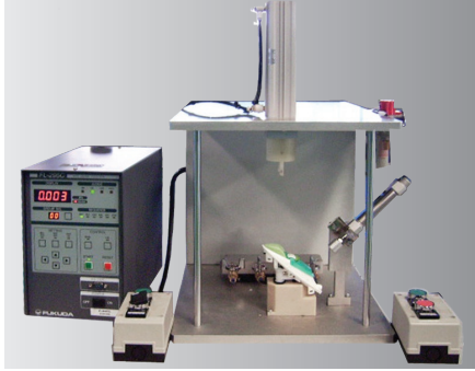
电熨斗安装件气密测试仪 Electric Iron Built-in Part leak tester
